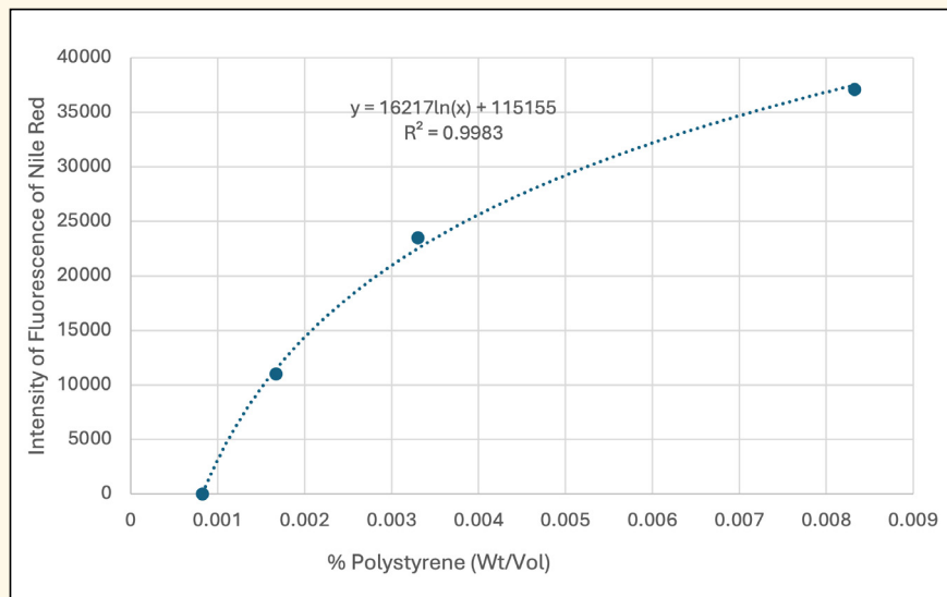
Figure 5: Standardized Curve of Fluorescence of Nile Red at Different Polystyrene Concentrations.
